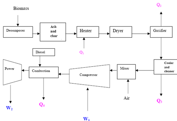
Figure 7: Advanced biomass power with diesel engine (Omer, 2006).
