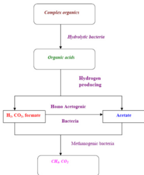
Figure 3: Biogas production process (Omer, 2003).
