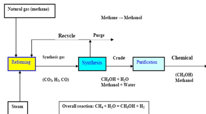
Figure 2: Schematic diagram shows methanol production (Omer, 2006).
